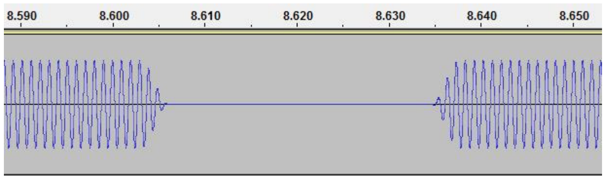
Figure 30: Sample-Rate Matcher underflow recovery — ring buffer half-filled with zeros.
