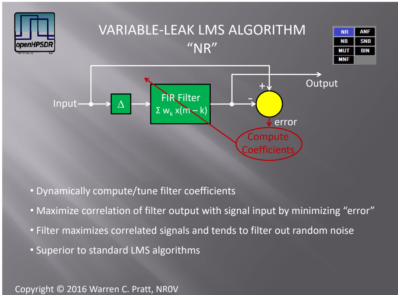
Figure 13: LMS Noise Reduction — adaptive filter structure separating noise-correlated and signal-correlated components.
