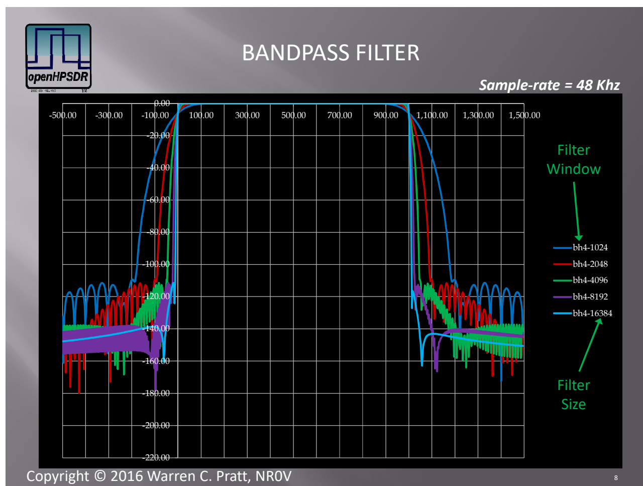
Figure 3: RXA Bandpass Filter frequency response, 4-term Blackman-Harris window, 48 kHz sample rate.
