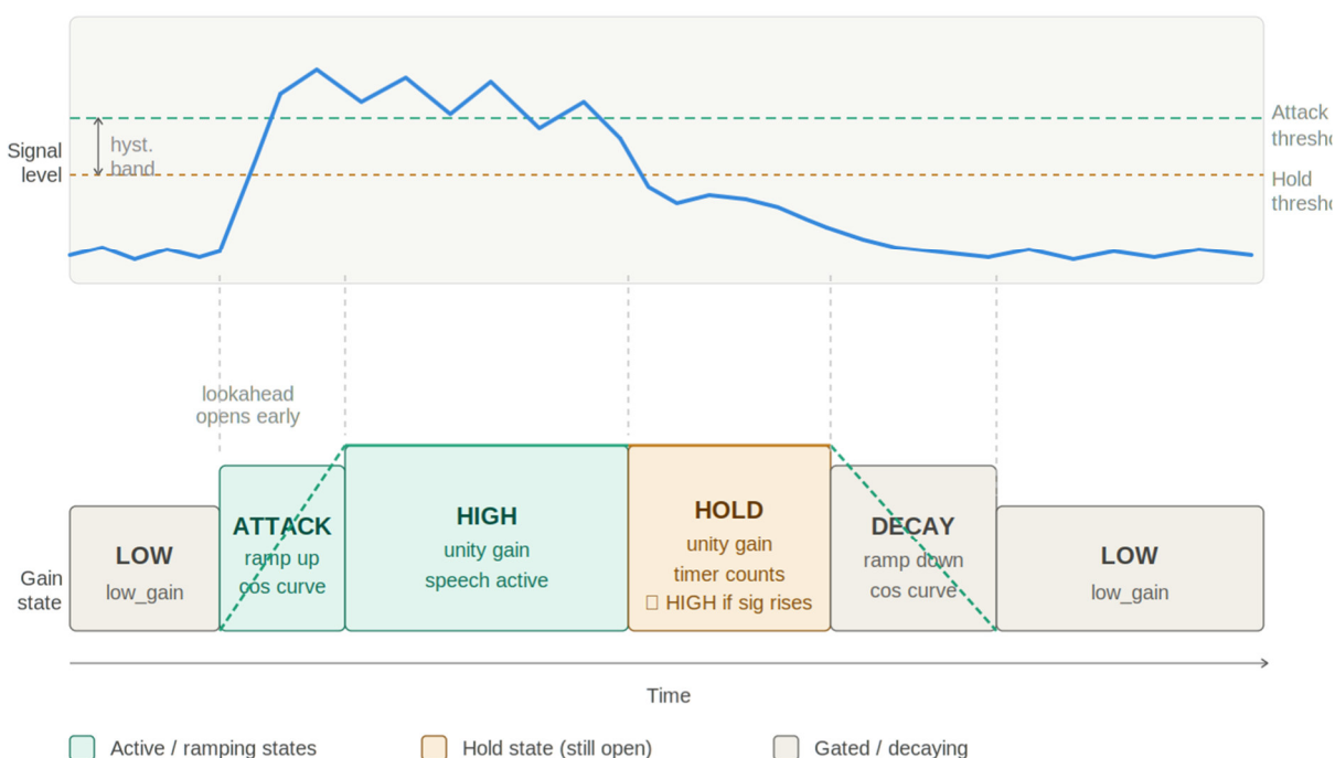
Figure C-3: DEXP state machine timeline. Upper track: input signal level versus the attack threshold (teal dashed) and hold threshold (amber dashed). Lower track: the five gain states and the raised-cosine gain transitions between them.
