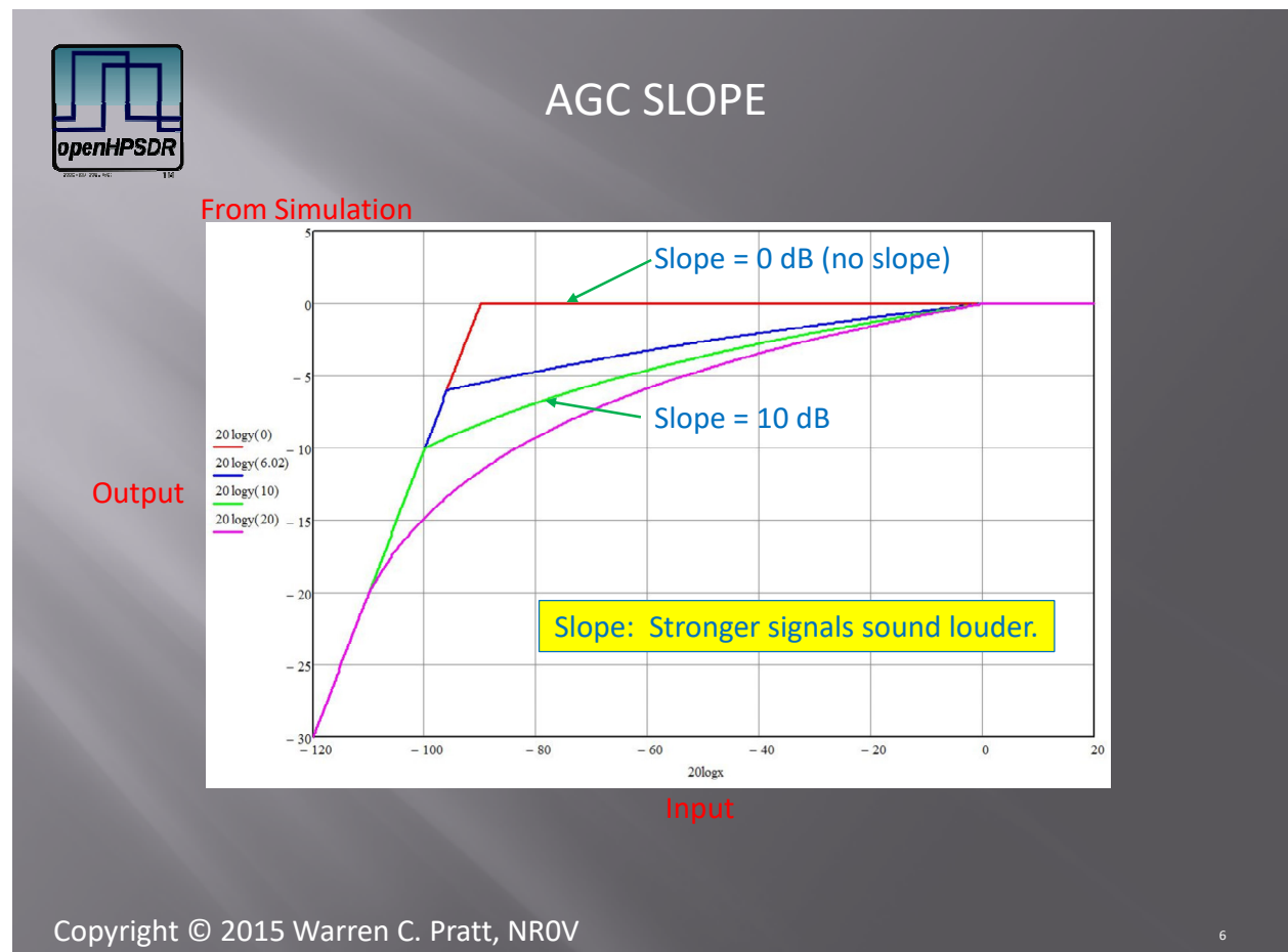
Figure 11: AGC Gain curve with slope values of 0, 6, 10, and 20 dB — output level versus input level.
