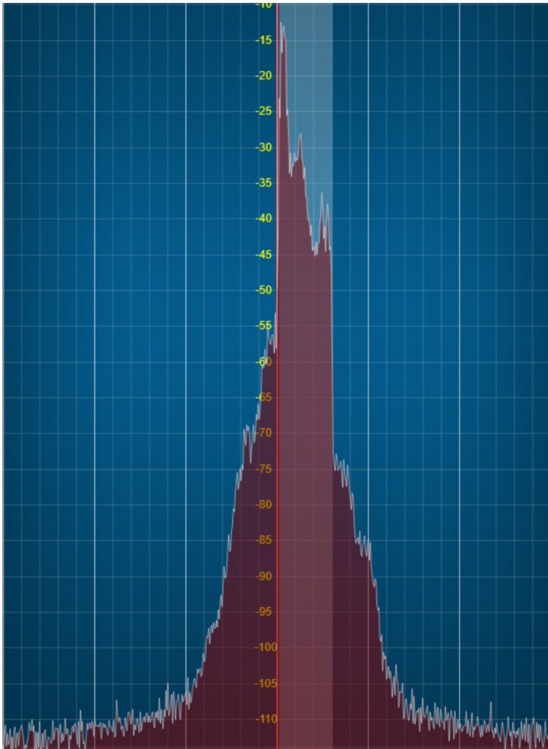
Figure C-7: Panadapter display of a transmitted SSB signal with adaptive predistortion DISABLED. The light-shaded area is the transmitted passband. IMD products are visible on both sides of the passband. The products to the left of the passband are not filter leakage — they are IMD products falling on that side of the signal.
