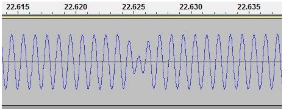
Figure 31: Sample-Rate Matcher overflow recovery — oldest half of ring buffer discarded.
