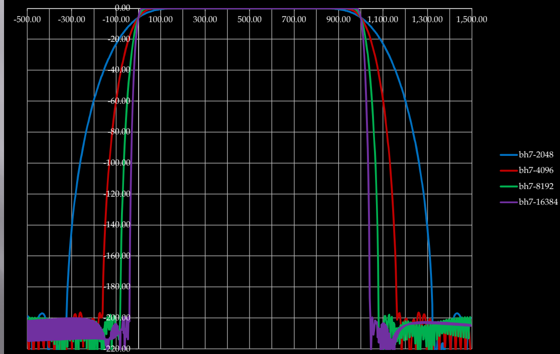
Figure 25: TXA Bandpass Filter frequency response, 7-term Blackman-Harris window, 96 kHz sample rate.
