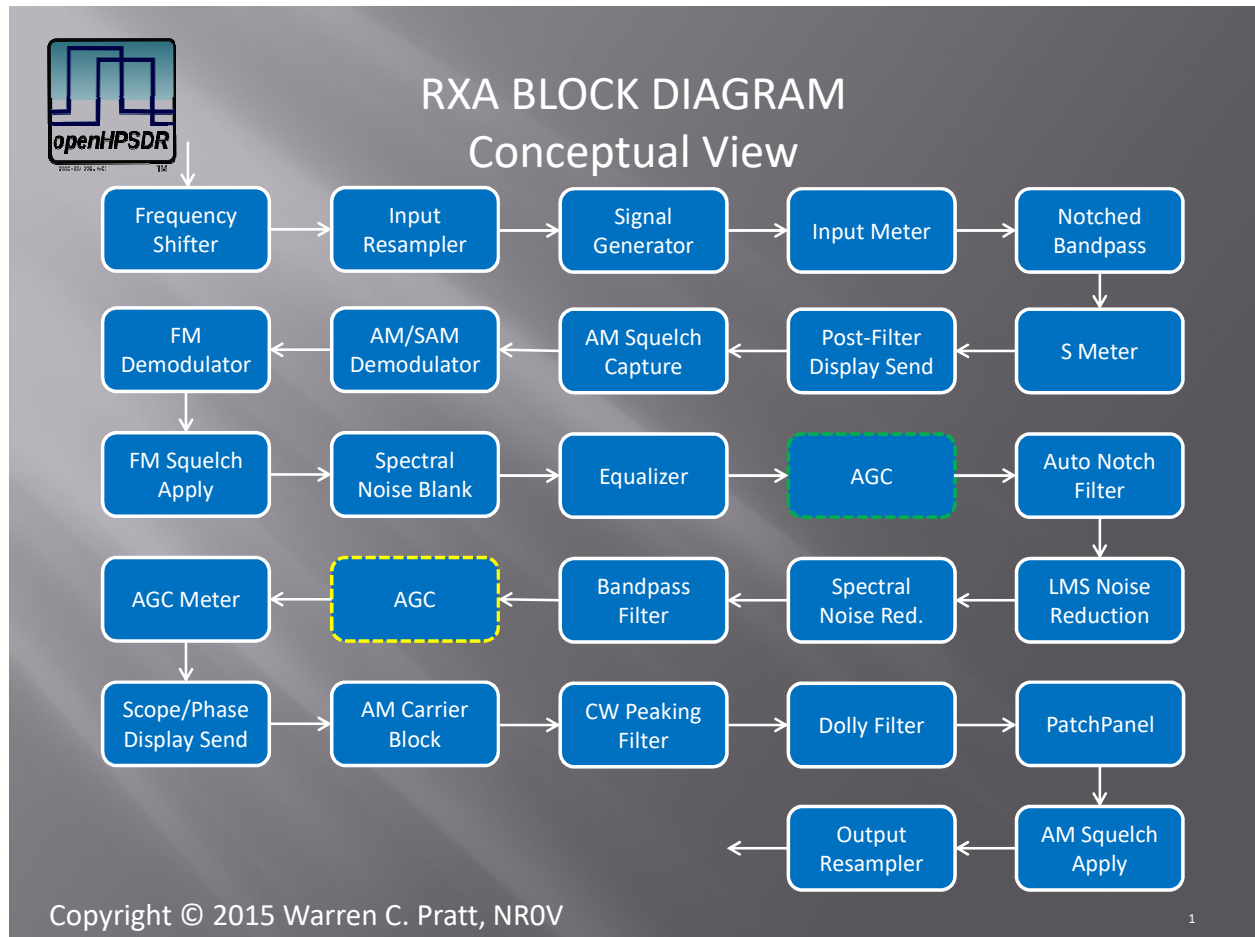
Figure 2: Block diagram of the RXA Receiver Unit showing the DSP processing chain.
