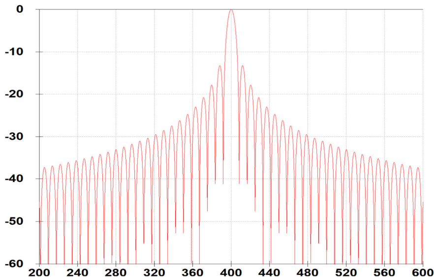
Figure 18: CW Peaking Filter — Matched Filter frequency response, optimized for maximum SNR.
