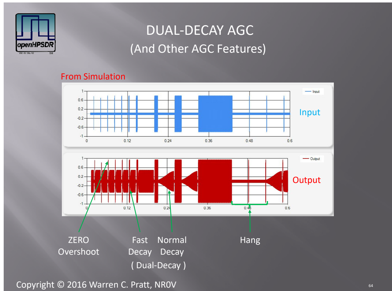
Figure 9: AGC Zero Overshoot, Dual-Decay, and Hang — independent fast and slow decay paths with hold period.
