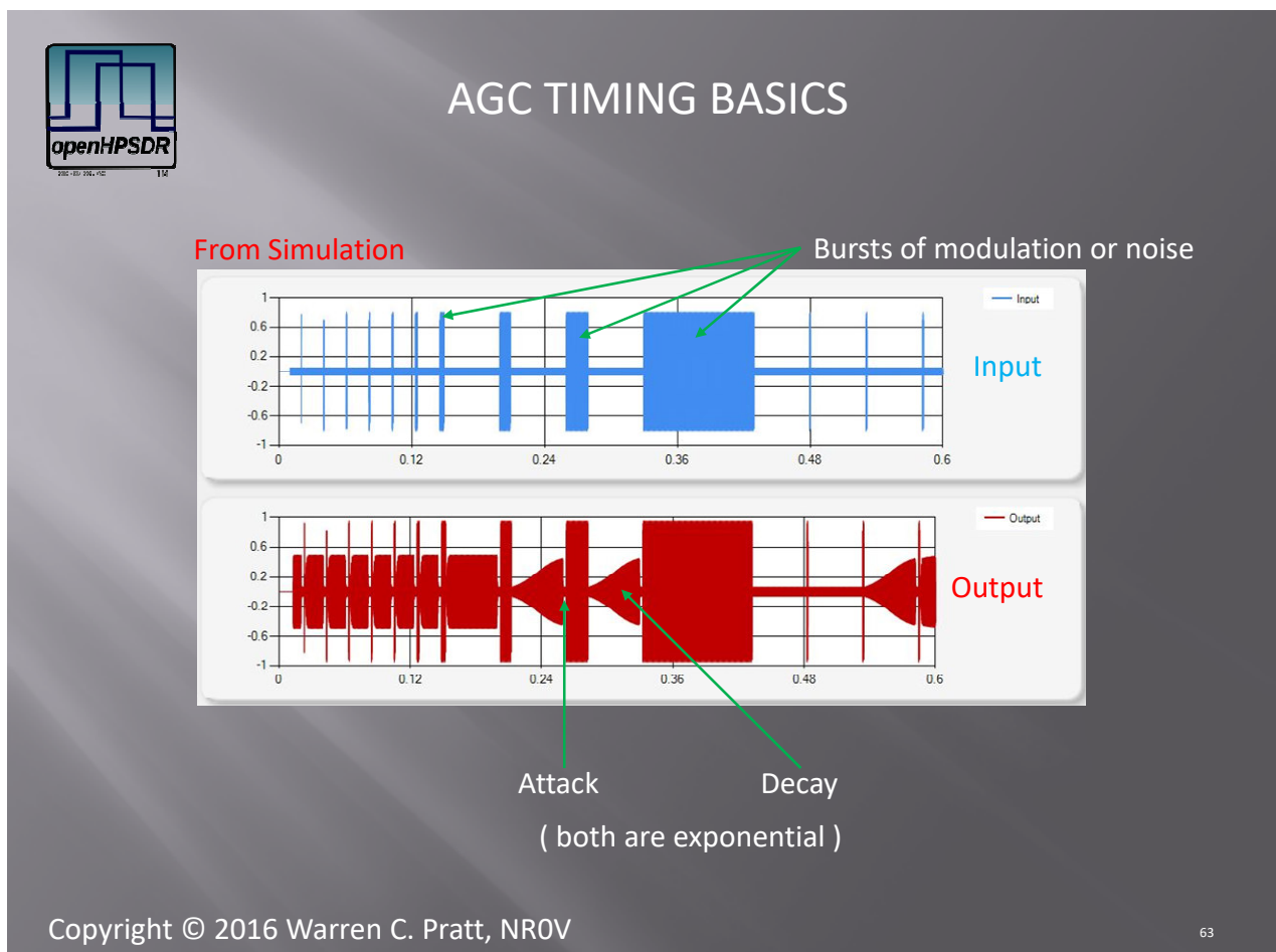
Figure 8: AGC exponential attack and decay waveforms illustrating attack and decay time-constant behavior.
