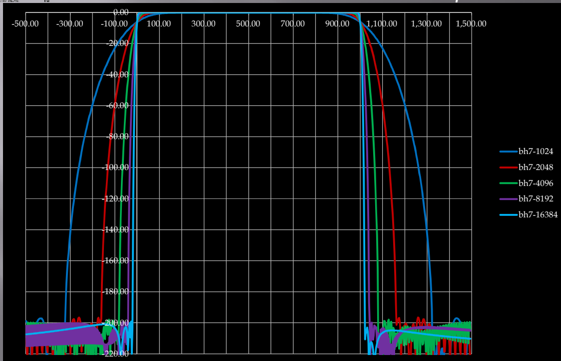
Figure 4: RXA Bandpass Filter frequency response, 7-term Blackman-Harris window, 48 kHz sample rate.
