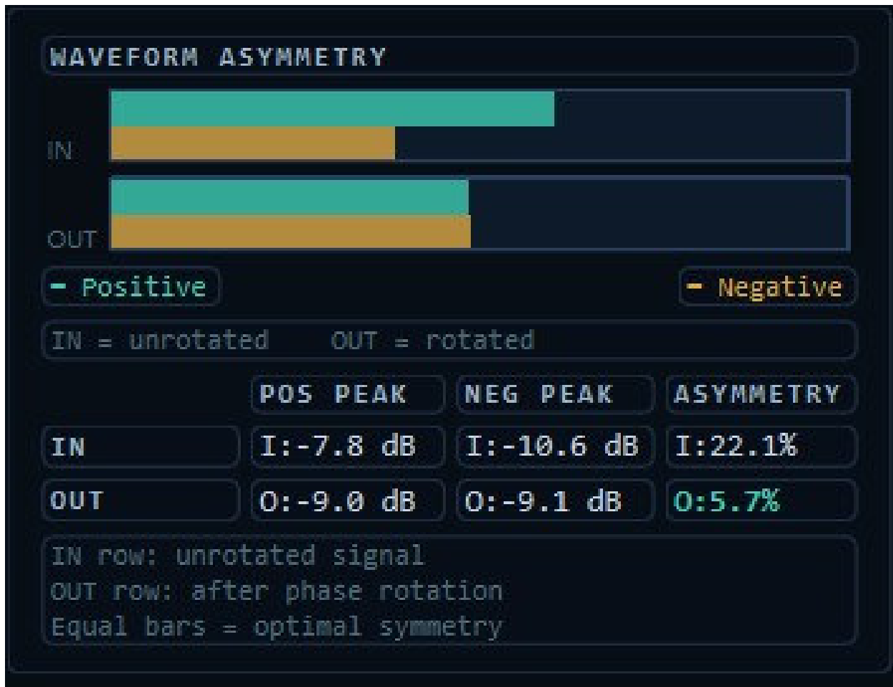
Figure C-2: Close-up of the Waveform Asymmetry display. IN row (unrotated): 22.1% asymmetry. OUT row (phase-rotated): 5.7% asymmetry — highlighted in teal when meaningfully better than the input.
