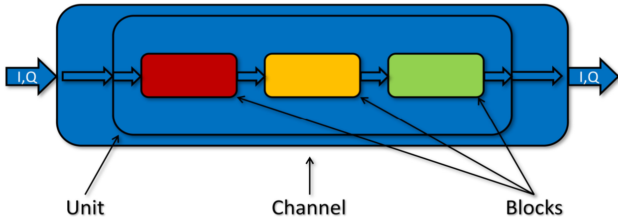
Figure 1: WDSP architecture overview — relationship between Channels, Units, and Blocks.
