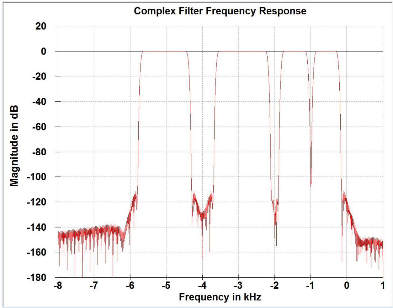
Figure 5: Example Notched Bandpass Filter with three notches at -1, -2, and -4 kHz relative to the tune frequency.
