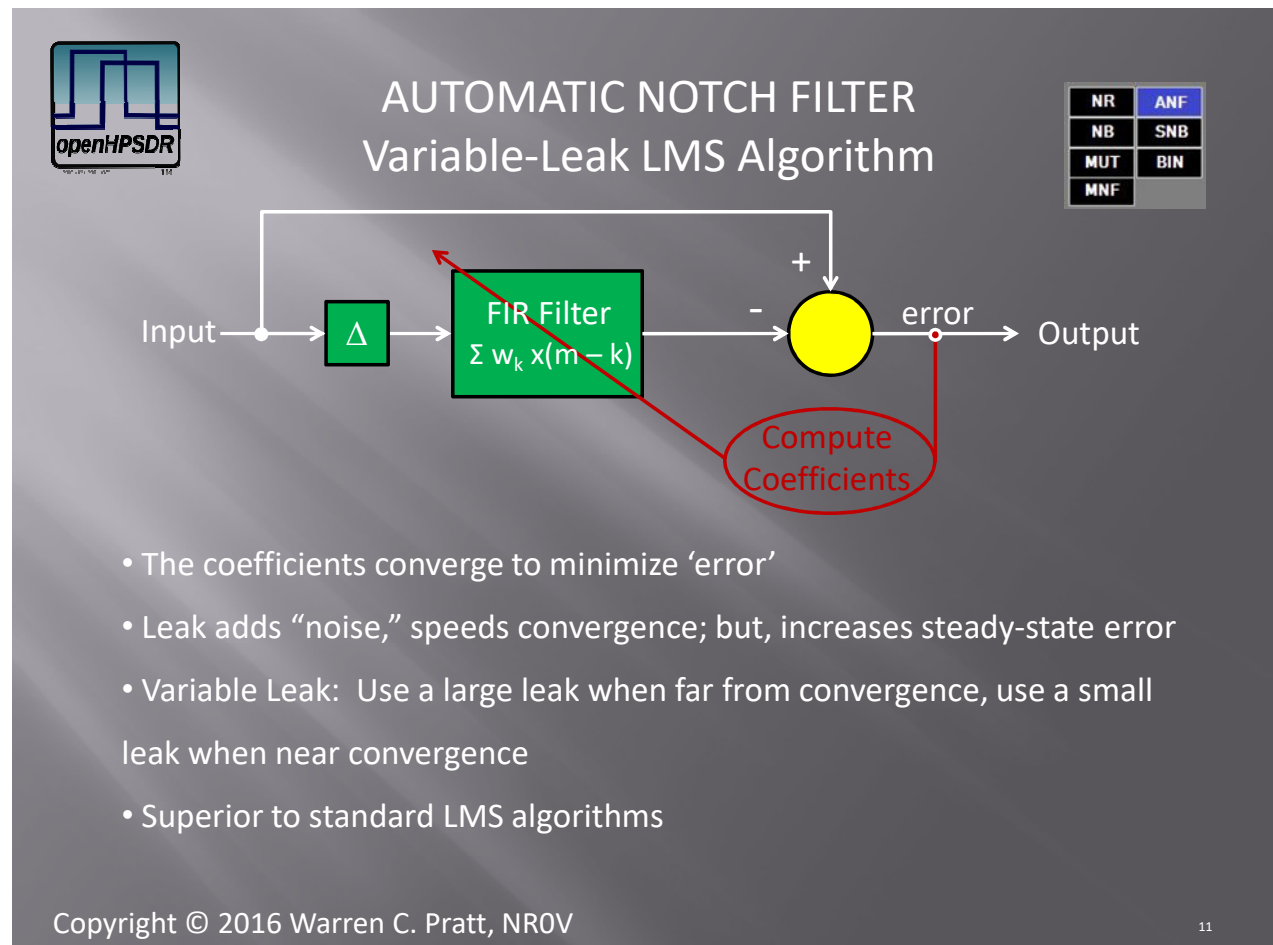
Figure 12: Automatic Notch Filter (ANF) — LMS adaptive filter tracking and removing a carrier from the passband.
