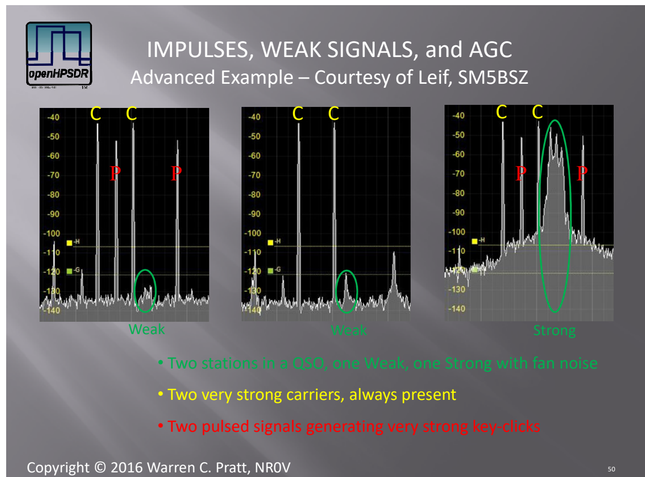
Figure 10: AGC Dual-Decay example showing frequency spectrum snapshots in the presence of two strong carriers.
