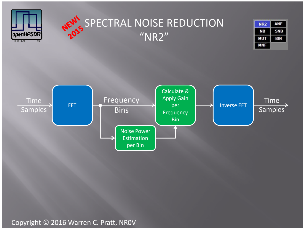
Figure 14: Spectral Noise Reduction — an implementation view.
