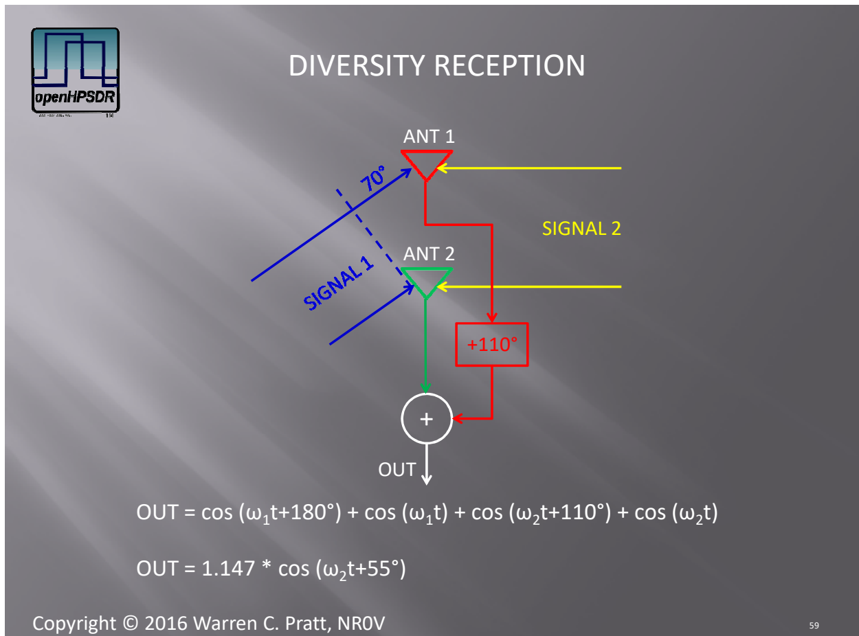
Figure 32: Diversity Mixer — two-antenna reception with adjustable phase and gain for signal combining.
