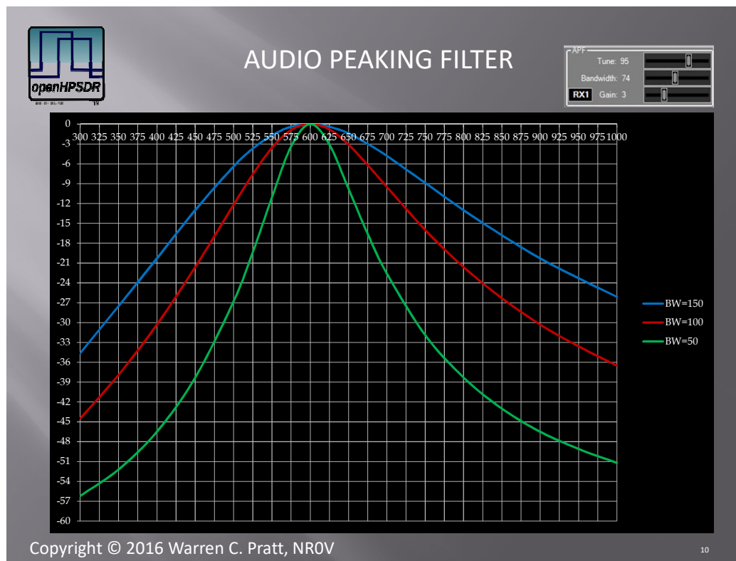
Figure 15: CW Peaking Filter — Bi-Quad (APF) frequency response centered at the CW signal frequency.
