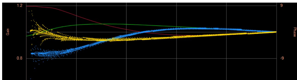
Figure 26: AmpView of amplifier with significant memory effects and a system with noisy data return. Blue – Magnitude input; Yellow – Phase input; Red – PureSignal magnitude correction; Green – PureSignal phase correction.
