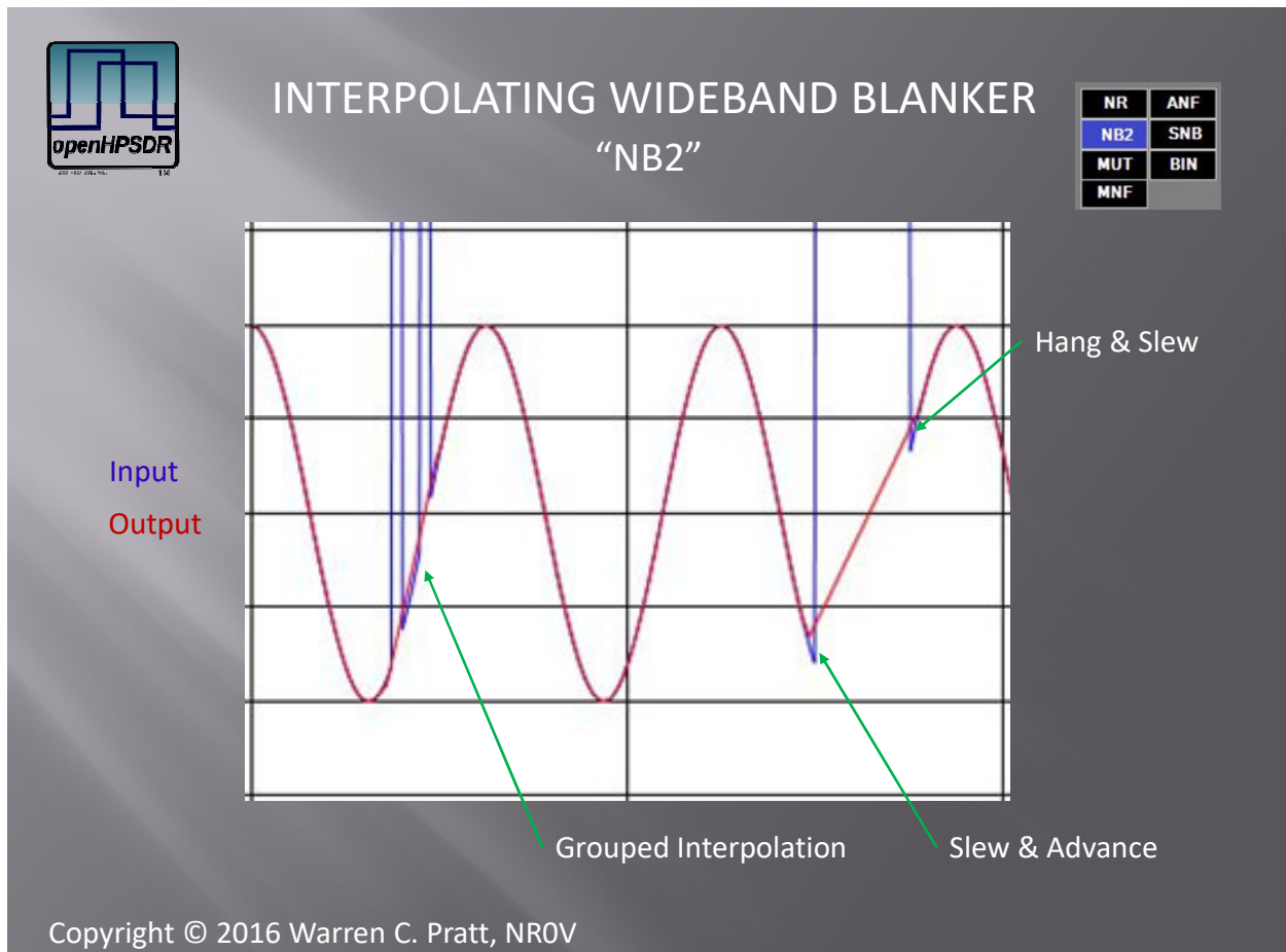
Figure 29: Interpolating Wideband Noise Blanker — impulse correction by interpolation across blanked samples.
