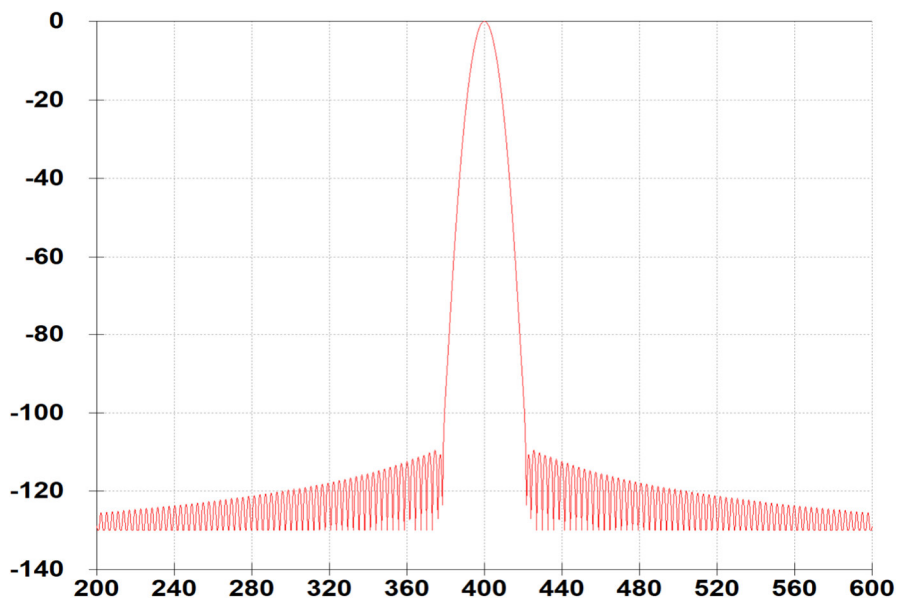
Figure 17: CW Peaking Filter — Gaussian frequency response showing zero-ringing rolloff.
