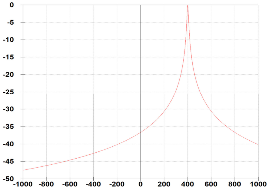
Figure 16: CW Peaking Filter — Double-Pole frequency response showing the sharper resonant peak.
