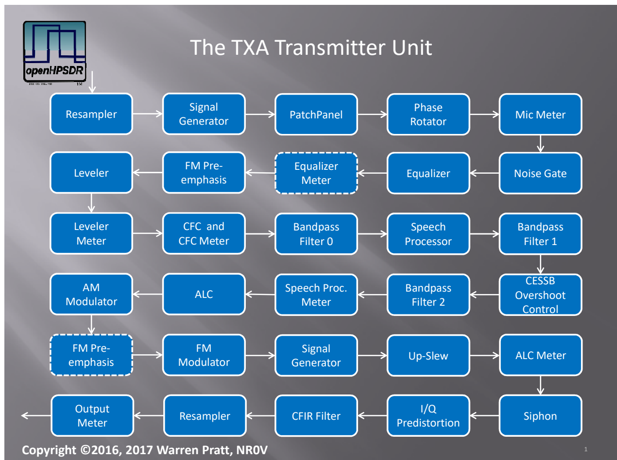
Figure 19: Block diagram of the TXA Transmitter Unit showing the transmitter processing chain.
